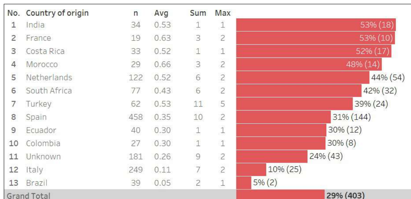
Figure 36. Countries of origin of imported products in Germany with the highest PFAS contamination in 2021.
