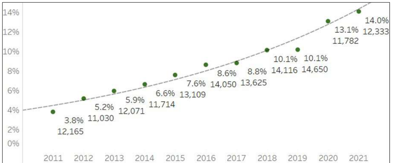
Figure 1. Average PFAS contamination in fruit sampled in the EU in the period 2011-2021.
